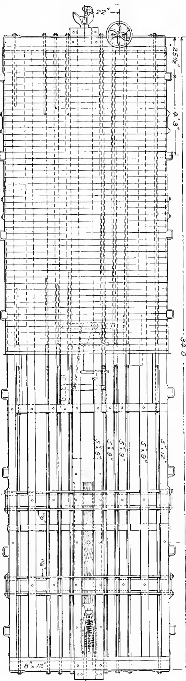
Fig. 291. Plan showing Floor and Underframing. FLAT-CAR BODY, CHICAGO & NORTH WESTERN RAILWAY. (Trucks are shown infra.) Capacity, 107,000 lb.
